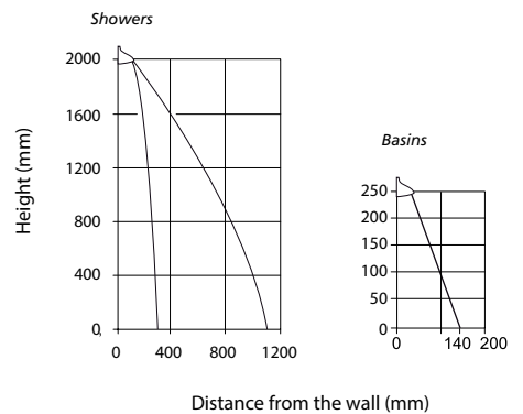
Spray Pattern at 200kPa
