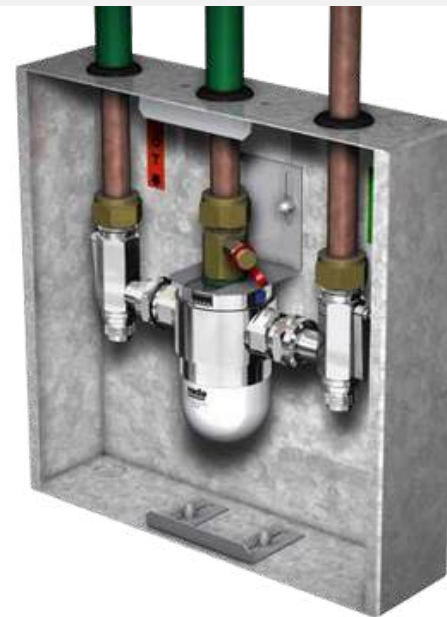
Rada 215dk in recessed 300mm galvanised box with stainless steel lid
