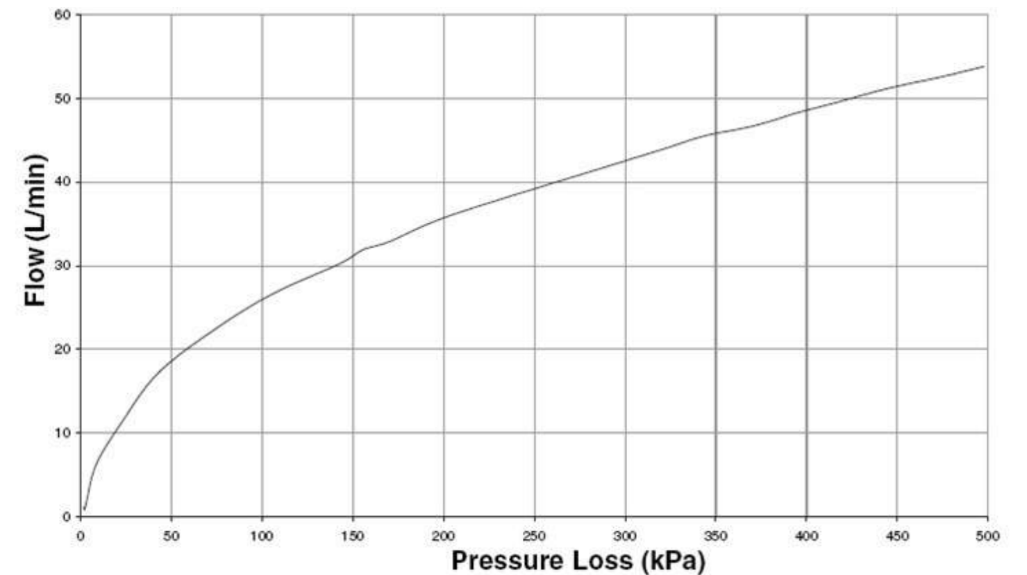
Flow Rate/Pressure Loss Graph
