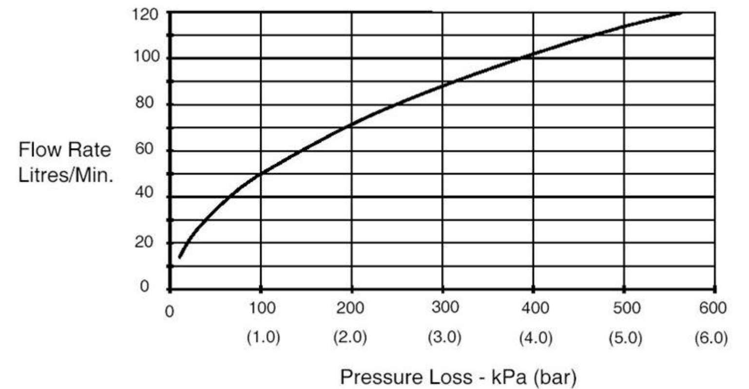
Flow Rate/Pressure Loss Graph
