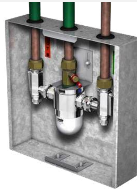
Rada 215dk in recessed box with lid
